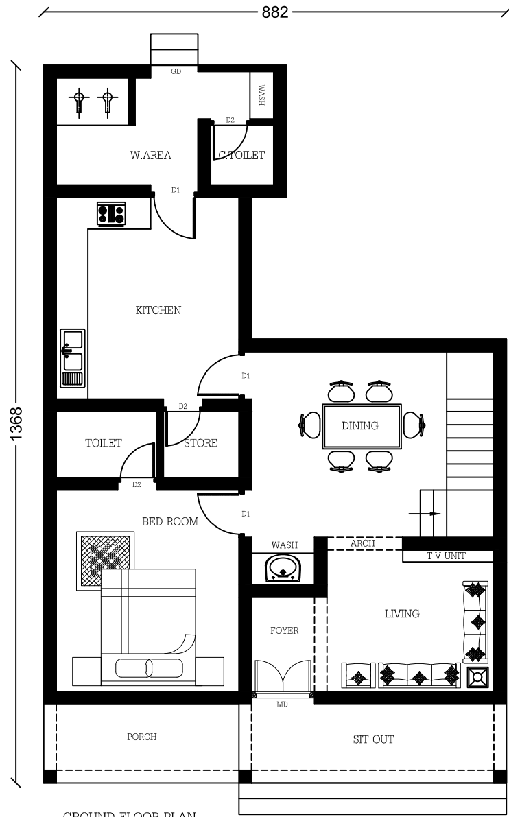
GROUND FLOOR PLAN G.F AREA = 1073 SQ FT G.F AREA = 697 SQ FT TOTAL AREA = 1770 SQ FT
