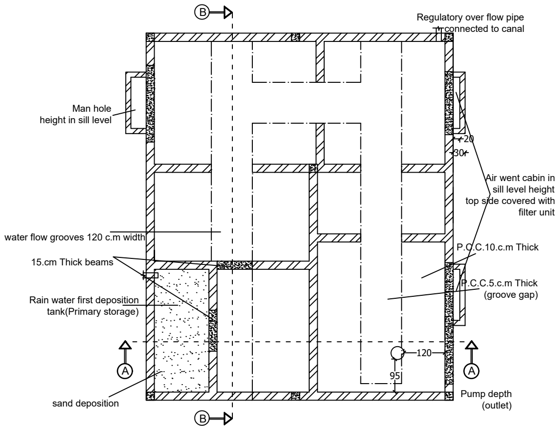
BASEMENT DETAIL PLAN
